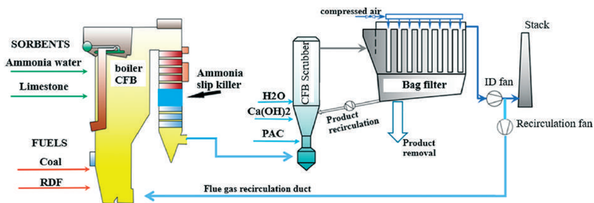
Figure 3. Graphic diagram of the CFB boiler system in connection with the FGT installation
