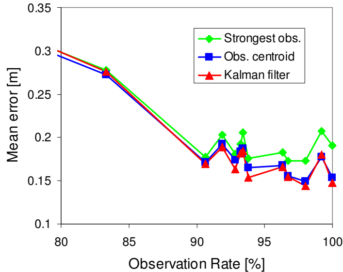
Figure 7. Positioning errors of the whole test group plotted as a function of observation rates.
